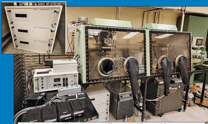
(3) VAC Vacuum Glove Boxes w/ Plasma Welding and Furnace Equipment
